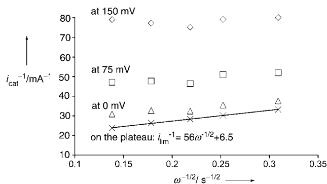
Figure 4. Dependence of the catalytic currents i_{\text{cat}} on O_2 flux (controlled by the electrode rotation frequency \omega ) as a function of the applied potential. [9] The solid line is a linear least-squares fit to the equation shown.
